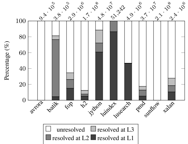
Figure 8: The percentages of invocations at non-inlined call sites for which the receiver type can be resolved using 1, 2, or 3 levels of calling context. Above each bar is the total number of invocations at non-inlined callsites.
