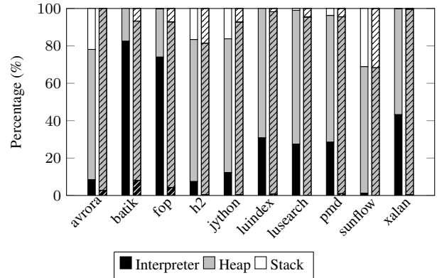
Figure 6: Proportions of allocation types for the 1st (without \text{\textbackslash} \text{\textbackslash} \text{\textbackslash} pattern) and the 15th (with \text{\textbackslash} \text{\textbackslash} \text{\textbackslash} pattern) benchmark iteration.
