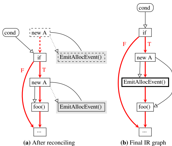
Figure 4: Base program IR with the associated ICGs after moving the allocation into the then-branch of the conditional, and after splicing the ICGs back into the base program IR. Dashed lines represent eliminated nodes and edges.
