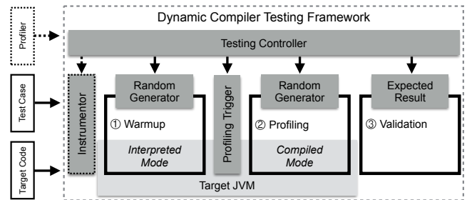
Figure 9: Overview of the dynamic compiler testing framework
