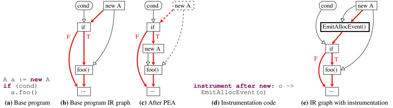
Figure 1: Instrumentation intercepting object allocations perturbing PEA due to dependency on the allocated object. In the IR graphs, rectangles represent fixed IR nodes, rounded rectangles represent floating IR nodes, thick red edges represent control flow, and thin black edges with hollow arrows represent data flow. Eliminated IR elements (nodes, control-flow edges, data-flow edges) are drawn using dashed lines.
