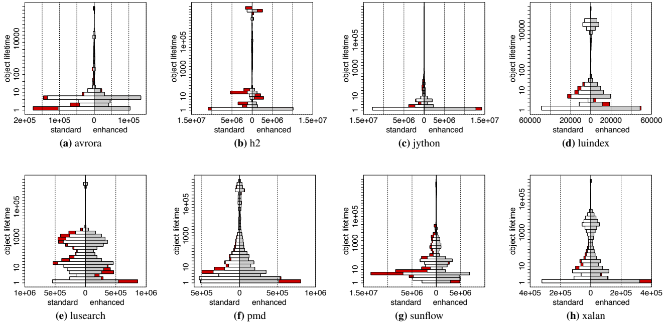
Figure 7: Back-to-back histogram of object lifetime distributions for the first benchmark iteration. The lifetimes are obtained using ET with the standard and the enhanced instrumentations. The X-axis denotes the object counts per bin. The differences between bins are marked in red. The results for the batik and the fop benchmarks are excluded due to less significant differences.
