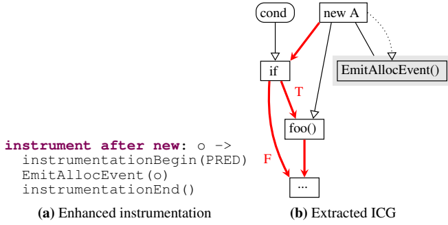
Figure 3: Enhanced instrumentation and the IR graph of the base program after extracting the instrumentation as an ICG. The gray rectangle in the IR graph represents an extracted ICG (the delimitation API invocations are omitted for clarity), solid black lines without arrows represent the association between an ICG and a base program node, and the dotted edges with hollow arrows represent a weak data-flow edge .
